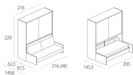
Kali Ponte Sofa 2561 braccioli/armrests cm 4-16
