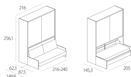
Kali Ponte Sofa 2561 braccioli/armrests cm 4-16
